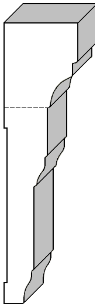
HDM HC555 (2 pcs: HC5 base & 55 brick) 1-5/16" x 5"
