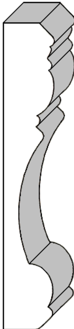
HDM 5B (beaded crown knife without back cut) 13/16" x 5-1/8"
